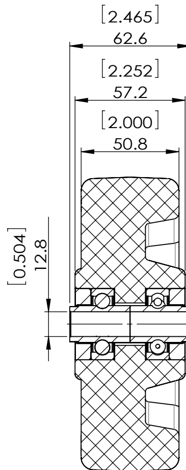
SECTION C-C
